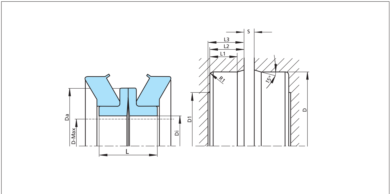
Figure 11 Installation Drawing
