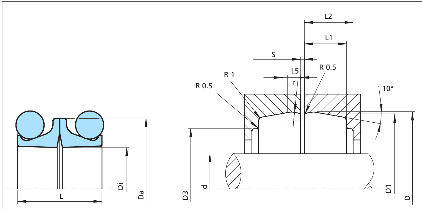
Figure 10 Installation Drawing
